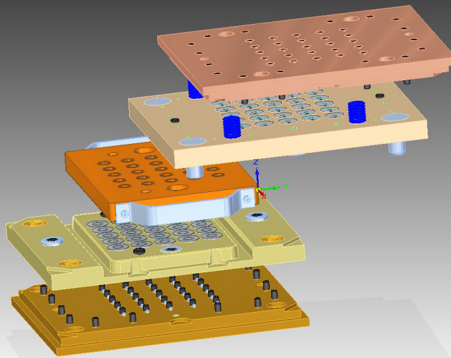
Exploded view of a die set capable of creating 20 diaphragms at once.
