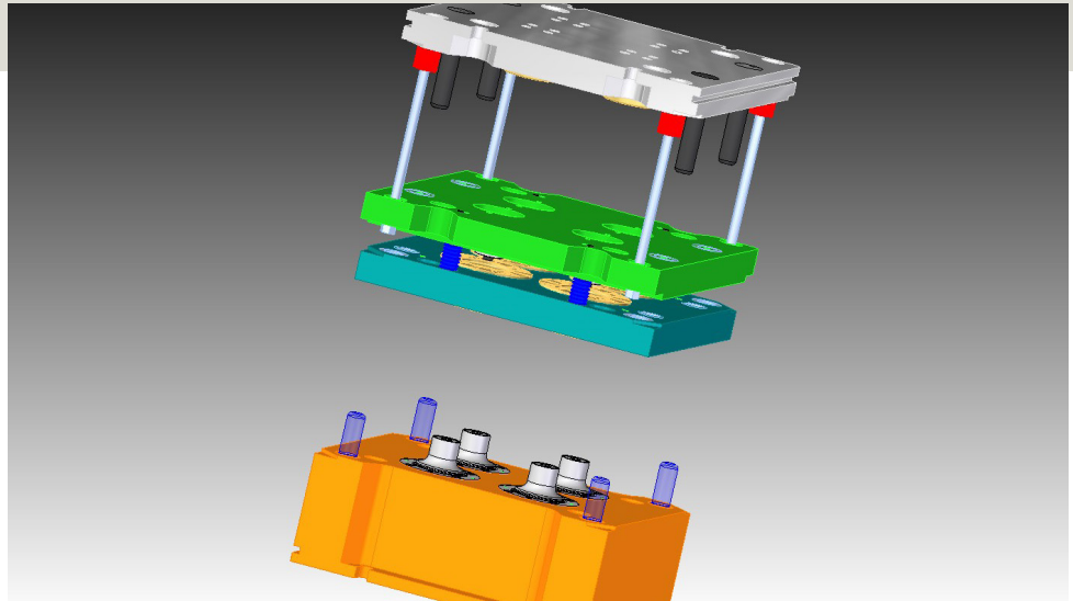
Die set that can form four diaphragms at once.
